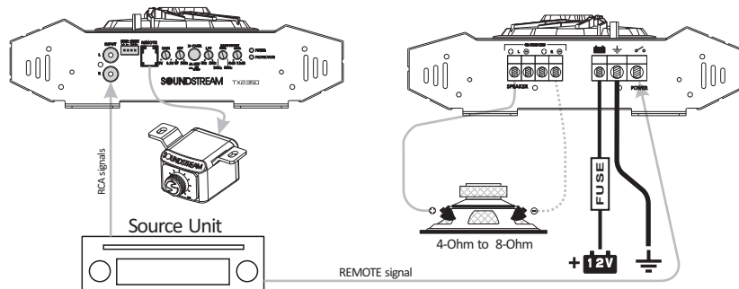
Fig 14. TX2.350 / TX2.500 wiring (High level input & Bridged mode)
