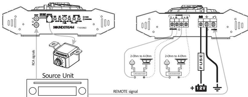
Fig 13. TX2.350 / TX2.500 wiring (2-channel mode)
