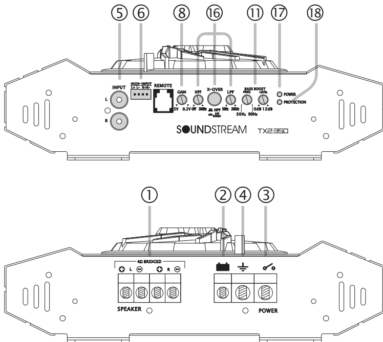
Fig 3. TX2.350/TX2.500 panel layout
