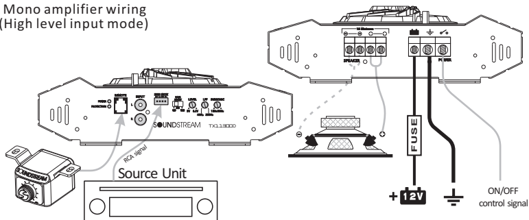
Fig 9. Mono amplifier wiring (multi woofers)
