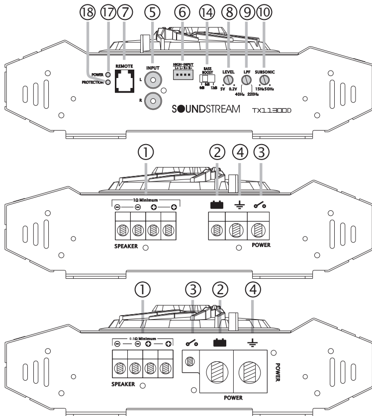
Fig 1. TX1.1300D/TX1.2000D/TX1.2600D Panel layout
