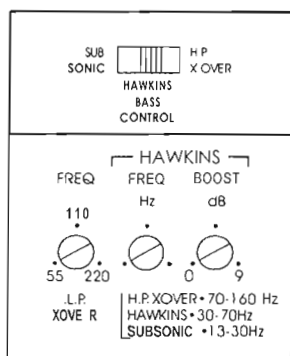
FIG. 1 BASS CONTROL
