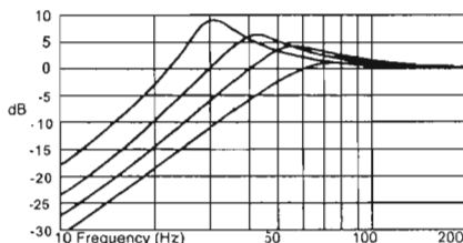
FIG. 6 VARIOUS SETTINGS
