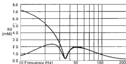
FIG. 5 LIMITED EXCURSION
