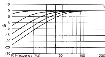
FIG. 3 VARIABLE HIGH PASS
