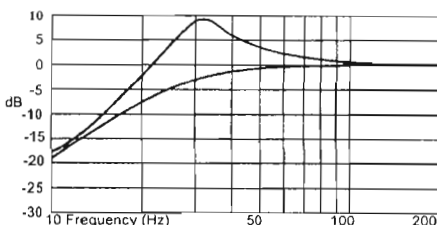
FIG. 2 VARIABLE "Q"
