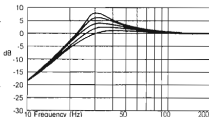
FIG. 2 VARIABLE BOOST
