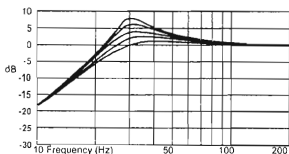
FIG. 4 VARIABLE BOOST
