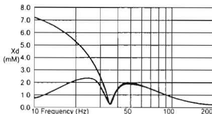
FIG. 3 Limited Excursion
