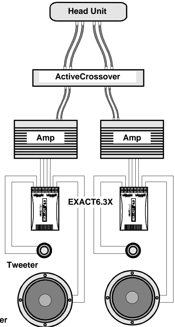
Figure 10 Active/Passive Bi-Amp
