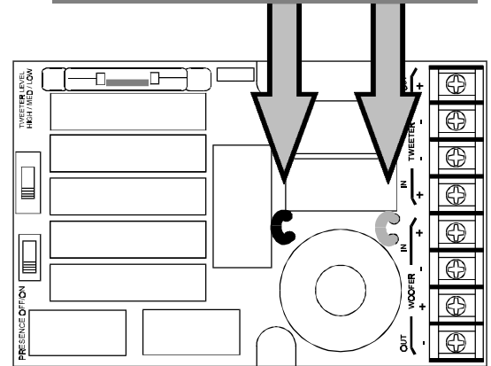
Figure 10 Active/Passive Bi-Amp
