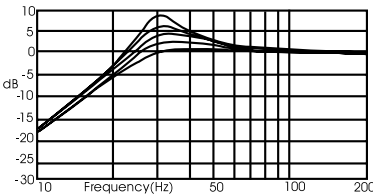
FIG. 4 VARIABLE BOOST
