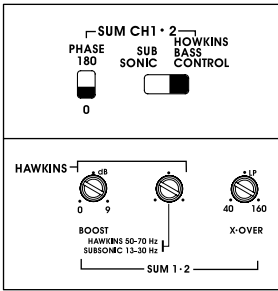
FIG. 1 BASS CONTROL
