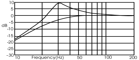
FIG. 2 VARIABLE "Q"
